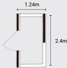
Dimensions (External) 1240mm D x 2400mm W x 2150mm H
