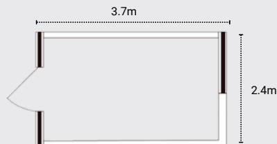
Dimensions (External) 3700mm D x 2400mm W x 2150mm H
